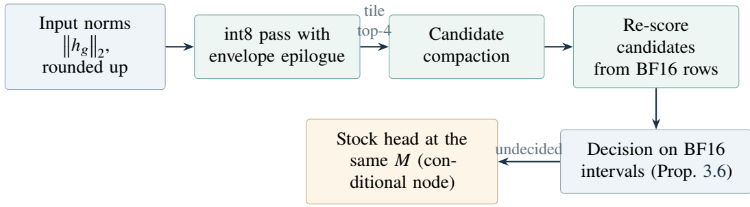
Figure 6: The certified greedy path. Only the approximate pass streams the whole head, in int8 at half the bytes of BF16; candidate rows are re-read in BF16, and the stock head runs only when the device-side flag is set.
