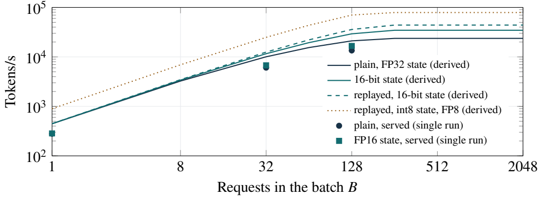
Figure 10: Derived throughput ceilings per lever stack against batch size (lines, evidence/moonshot/ceilings.csv ) and served output throughput of single benchmark runs at client concurrency 1, 32 and 128 (points, evidence/moonshot/lever_sweeps_quick.csv ). The gap between line and point at a given concurrency is overhead above the byte-and-arithmetic floor, and at high concurrency it includes the server’s streaming path.
