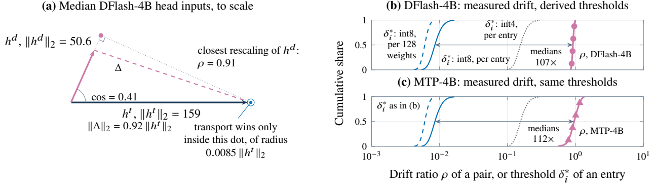
Figure 4. Why transport fails. (a) Median DFlash-4B head inputs, to scale: norms over the 4,020 transport pairs, cosine over 20,000 random drift pairs. Transport’s bound beats the int8 copy’s only if h^d lies in the dot at the tip of h^t , of radius \delta^* \|h^t\|_2 for the median \delta^* (Proposition 5.2). (b, c) Cumulative distributions of the measured drift \rho over 40,000 aligned held-out pairs of DFlash-4B (b) and MTP-4B (c), against the thresholds \delta_i^* derived from the weights for every vocabulary entry (64-entry tiles of contiguous token indices); the arrows join the median threshold for int8 with one scale per entry to each drafter’s median drift (107 and 112 times apart) [E21,E22,E23,E25,E26].
