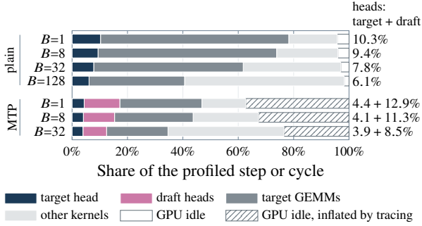
Figure 1. Where the GPU time of a stock decode step goes (baseline; no certified head), measured under Nsight Systems with a fixed number B of requests per decode step [E41]; in plain decoding, each head call then has M = B positions. The target head is its GEMM, the FP32 copy of its logits and the argmax. An MTP cycle adds the drafter’s heads. The numbers beside the bars give the heads’ share: the target head for plain decoding, target plus drafter heads for MTP. Tracing lengthens the host-bound MTP cycle’s idle time (hatched) but barely changes kernel durations, so the heads’ shares of an untraced cycle are larger than shown (Appendix E.2).
