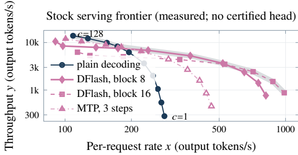
Figure 5. Stock serving frontier (baseline; no certified head): four of nine tuned arms, client concurrency 1 (lower right) to 128 (64 for 16-token DFlash blocks). Points average three or four sessions (hollow: one); one standard deviation, below 2% of each mean, hides behind the markers [E48]. Grey: envelope of all nine arms’ points with three or more sessions.
