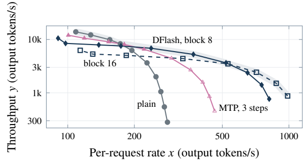
Figure 5. The confirmed serving frontier, one curve per tuned arm from client concurrency 1 (lower right) to 128 (upper left); each point is the mean of three server sessions on the confirmation split (hollow: one) [E67]. Grey: the envelope of the three-session points. Every arm is stock or exact up to rounding; none uses the certified head.
