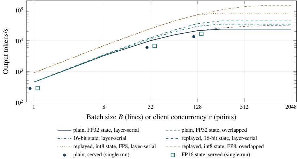
Figure 6. Derived throughput ceilings per lever stack against batch size under the layer-serial model of Equation (11) and, for two stacks, the overlapped roofline of Equation (12), at the measured bandwidth and assumed tensor-core rate (lines [E33]), and served output throughput of single benchmark runs at client concurrency 1, 32 and 128 (points [E34]; the two series are offset slightly left and right of their concurrency so that both stay visible). The gap between a line and a point at the same concurrency is overhead above the layer-serial floor; at high concurrency it includes the server’s streaming path (Appendix E.8).
