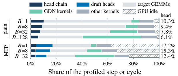
Figure 1. GPU time of a decode step by component, measured under Nsight Systems at a fixed batch B [E39]; an MTP cycle (three draft steps) commits several tokens. Right: the heads’ share of the profiled step or cycle. Tracing inflates the MTP cycle’s idle time; untraced it is about 21%, 20% and 15% (derived, Appendix E.2).
