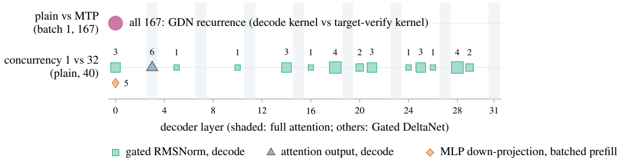
Figure 7. Where equivalent stock configurations first produce different module outputs, by decoder layer. Plain decoding and MTP speculation part at layer 0’s GDN recurrence in every prompt, because decode and target verify use different recurrent kernels. Plain decoding at concurrency 1 and 32 (batches of up to 16) part at batch-dependent kernels spread over the depth: the gated RMSNorm of GDN layers (marker size and label give the count), layer 3’s attention, or layer 0’s MLP in a batched prefill. For plain decoding against MTP, a rerun of 40 prompts that also hashes the caches finds every cache entering the differing recurrence identical; for the concurrency pair these are first differing module outputs only, and whether the caches entering them agree is pending. Each pair’s two tapped servers had different pools. Measured with a bit-exact tap [E32, E35].
