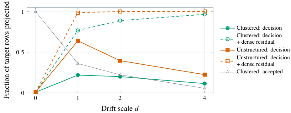
Figure 6. Work counts on constructed heads, not timings [E29]. Solid lines count the rows needed to decide acceptance; dashed lines add a dense residual completion after each rejection. The thin line is the fraction of proposals accepted in the clustered family. Evidence production, bounds, bonus sampling and the backbone are excluded.
