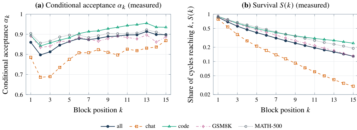
Figure 9. The public DFlash drafter by block position, block size 16, greedy with thinking on, per domain of the panel. (a) Conditional acceptance \alpha_k ; (b) the share of verify cycles that accept at least k drafted tokens, on a logarithmic axis. Measured in correctness runs [E59]; the late rise in (a) is a selection effect of the few cycles that get that far.
