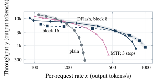
Figure 5. The confirmed serving frontier for four of the nine tuned arms, from client concurrency 1 (lower right) to 128, or 64 for block 16 (upper left); each point averages its valid sessions (three or four; hollow: one) [E78]. Grey: the envelope over all nine arms’ points with at least three sessions. All arms are stock or exact up to rounding; none uses the certified head.
