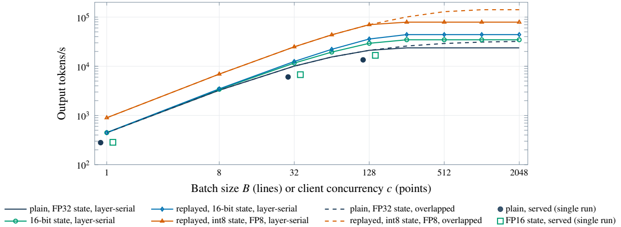
Figure 8. Derived throughput ceilings per lever stack against batch size under the layer-serial model of Equation (11) and, for two stacks, the overlapped roofline of Equation (12), at the measured bandwidth and assumed tensor-core rate (lines [E45]), and served output throughput of single benchmark runs at client concurrency 1, 32 and 128 (points [E46]; the two series are offset slightly left and right of their concurrency so that both stay visible). The gap between a line and a point at the same concurrency is overhead above the layer-serial floor; at high concurrency it includes the server’s streaming path (Appendix E.8).
