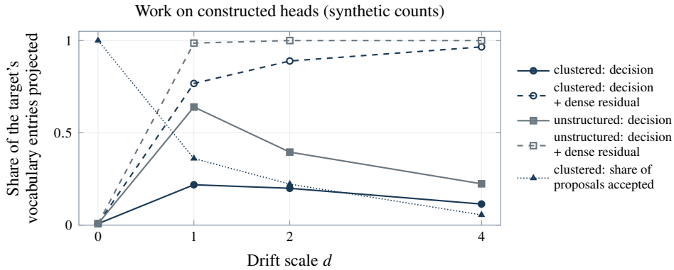
Figure 3. Work counts on constructed heads, not timings [N-E18]. Solid lines count the rows needed to decide acceptance; dashed lines add a dense residual completion after each rejection. The dotted line is the share of proposals accepted in the clustered family. Evidence production, bounds, bonus sampling and the backbone are excluded.
