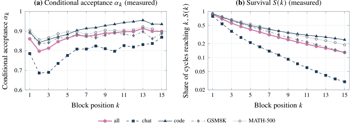
Figure 2. The public DFlash drafter by block position, block size 16, greedy with thinking on, per domain of the panel. (a) Conditional acceptance \alpha_k ; (b) the share of verify cycles that accept at least k drafted tokens, on a logarithmic axis. Measured in correctness runs [N-E51]; the late rise in (a) is a selection effect of the few cycles that get that far.
