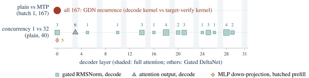
Figure 5. Where equivalent stock configurations first produce different module outputs, by decoder layer. Plain decoding and MTP speculation part at layer 0’s GDN recurrence in every prompt, because decode and target verify use different recurrent kernels. Plain decoding at concurrency 1 and 32 (batches of up to 16) part at batch-dependent kernels spread over the depth: the gated RMSNorm of GDN layers (marker size and label give the count), layer 3’s attention, or layer 0’s MLP in a batched prefill. For plain decoding against MTP, a rerun of 40 prompts that also hashes the caches finds every cache entering the differing recurrence identical; for the concurrency pair these are first differing module outputs only, and whether the caches entering them agree is pending. Each pair’s two tapped servers had different pools. Measured with a bit-exact tap [E23, E26].
