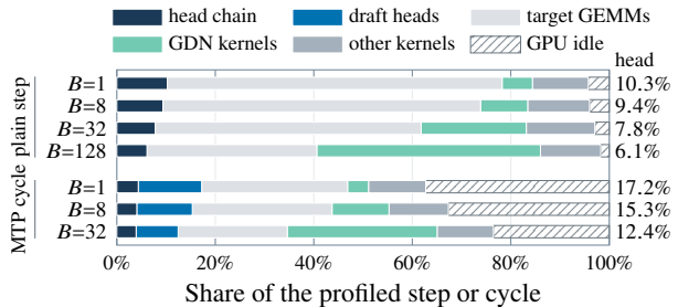
Figure 1. GPU time of a decode step by component, measured under Nsight Systems at a fixed batch B [E30]; an MTP cycle (three draft steps) commits several tokens. Right: the share of the target and draft heads, which bounds what a free head could save; it falls as the Gated DeltaNet kernels grow with B .
