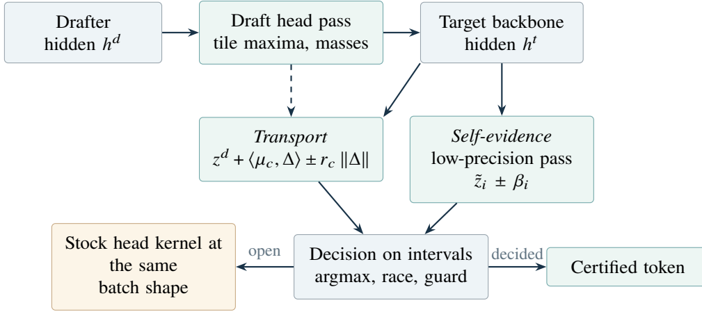
Figure 1: Two sources of evidence for the same decision. Transport reuses the drafter’s head pass and bounds only the change \Delta = h' - h^d ; self-evidence pays for a cheap pass over the head at the target state. Either way the decision is taken on intervals, rows or tiles are refined while it stays open, and a row that cannot be certified runs the stock head kernel. The target backbone always runs; the saving, if any, is in the head.
