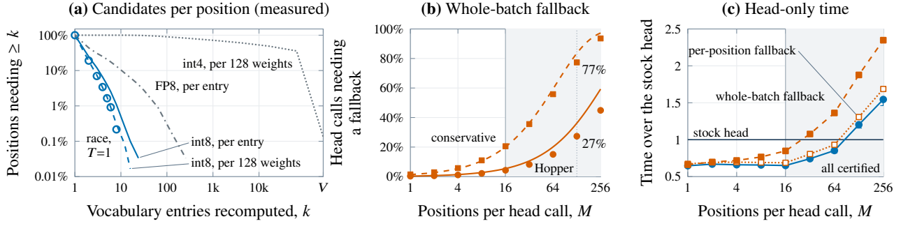
Figure 3. Int8 leaves few candidates, but whole-batch fallback grows with the batch; timed alone, with the per-position fallback under the conservative model, the head is expected to take about 0.7 of the stock head’s time up to 16 positions, and every mode is slower from 128. (a) Held-out replay, R-real: four copies, greedy, and the per-128-weights int8 copy in a seeded race at T = 1 [E4]. (b) Lines: independent fallback at Table 6’s held-out shares [E6]; markers: kernel replay [E17]. (c) Over the stock head: measured with every position certified (medians; p10–p90 within the markers below 256), and expected with each fallback, from measured times and (b)’s conservative rates [E17]. Shaded: consecutive replay positions, not engine batches.
