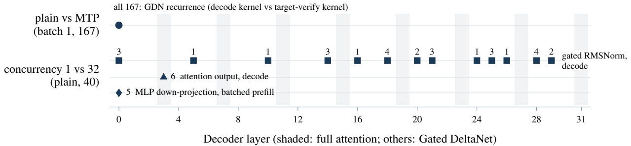
Figure 6. Equivalent stock configurations first differ upstream of the head: plain decoding and MTP at layer 0’s GDN recurrence in every prompt, because decode and target verify use different recurrent kernels, and plain decoding at concurrency 1 and 32 (batches of up to 16) at batch-dependent kernels across the depth. Each number counts the prompts at its mark. The plotted runs’ two tapped servers had different pools in each pair. Reruns of 40 prompts that also hash the caches find them identical on entry: for plain decoding against MTP, every cache entering the differing recurrence; for the concurrency pair, with identical fixed pools, every cache entering every forward up to the first differing module output (gated norm 30, layer 3’s attention 5, batched-prefill down-projection 5, against 29, 6 and 5 plotted). Measured with a bit-exact tap [E33,E36].
