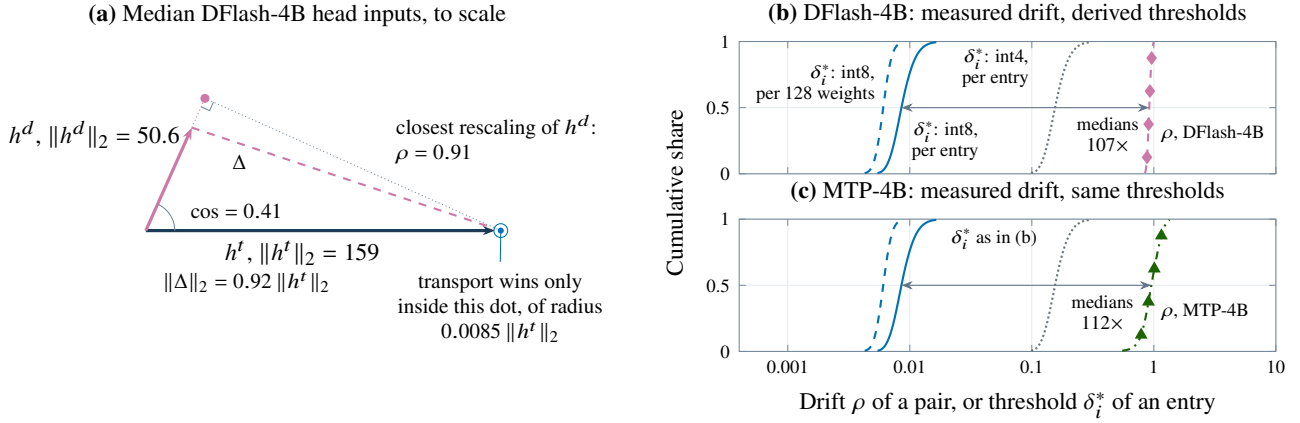
Figure 5. Transport fails because draft head inputs are far from the target’s: the median drift is 107 (DFlash-4B) and 112 (MTP-4B) times the median threshold \delta^* below which transport beats the per-entry int8 copy. (a) Median DFlash-4B head inputs, to scale (norms over the 4,020 whole-step pairs, cosine over 20,000 random aligned pairs); transport wins only if h^d lies in the dot of radius \delta^* \|h^t\|_2 (Proposition 5.2). (b, c) Drift \rho over 40,000 aligned held-out pairs per drafter, against each entry’s threshold \delta_i^* from the weights; arrows join the medians [E21,E22,E23,E25,E26].
