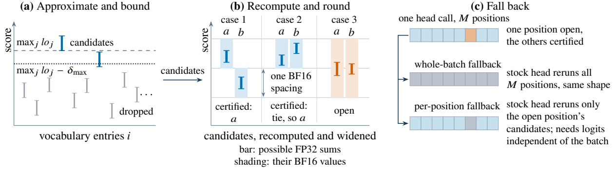
Figure 2. The certified head drops every entry that cannot win, recomputes the few that remain, and falls back to the stock head when the token stays open (schematic; values illustrative). (a) The int8 copy bounds each entry’s exact score by [lo_i, hi_i] ; an entry with hi_i < \max_j lo_j - \delta_{\max} cannot win; \delta_{\max} covers the stock kernel’s modelled error and rounding (Section 2.2). (b) Three candidate pairs a, b , recomputed from BF16 weights and widened to the FP32 sums the stock kernel could form. (c) The two fallbacks (Section 2.3).
