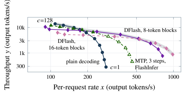
Figure 4. Under SGLang’s default admission, speculation leads plain decoding at low concurrency and trails it at high: the best arm of each drafter (not all drawn) serves more up to c = 32 and less from 48. Four of nine tuned stock arms, c = 1 to 128 (64 for 16-token DFlash); points average three or four sessions (hollow: one), with standard deviations under 2% of each mean [E50]. Grey: Pareto envelope of all nine arms’ points with three or more sessions.
