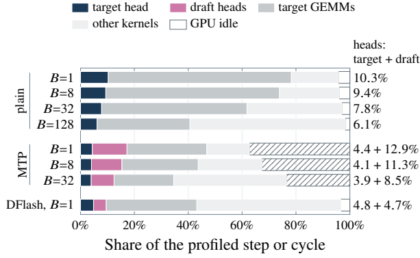
Figure 1. Where the GPU time of a stock decode step goes (measured under Nsight Systems; baseline, no certified head), with a fixed number B of requests per decode step, so that a head call in plain decoding has M = B positions [E41]. The target head comprises its GEMM, the FP32 copy of its logits and the argmax. Tracing inflates the MTP cycle’s idle time (hatched) but barely changes kernel durations, so the MTP heads’ shares of an untraced cycle are larger than shown (Appendix E.2). DFlash: the tuned arm with 16-token blocks, which is GPU-bound [E45].
