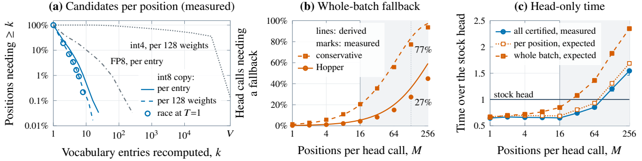
Figure 3. What the certified head costs. (a) Held-out replay, R-real decision: share of positions that need at least k candidates, for four copies of the head (greedy) and for the int8 copy with one scale per 128 weights in a seeded race at T = 1 [E4]. (b) Share of head calls of M positions that fall back to the stock head: lines if positions fell back independently at the held-out shares of Table 6 [E6]; markers from the kernel replay [E17]. (c) Time per call over the stock head’s, head alone: measured with every position certified (medians; p10–p90 within the markers below 256), and expected with each fallback under the conservative model from measured times and the rates of (b) [E17]. Shaded: above 16 positions the calls are consecutive replay positions, not engine batches.
