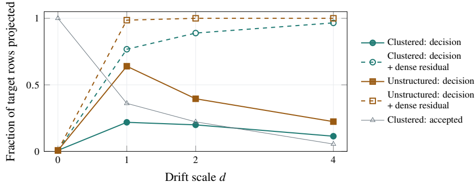
Figure 4. Work counts on constructed heads, not timings [E20]. Solid lines count the rows needed to decide acceptance; dashed lines add a dense residual completion after each rejection. The thin line is the fraction of proposals accepted in the clustered family. Evidence production, bounds, bonus sampling and the backbone are excluded.
