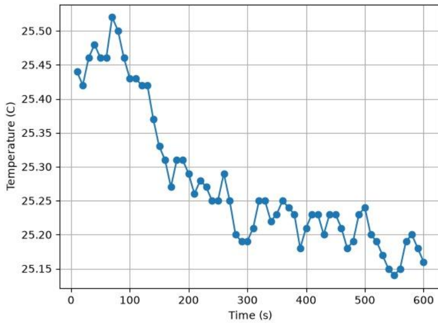
Figure 2: Temperature measurement results
