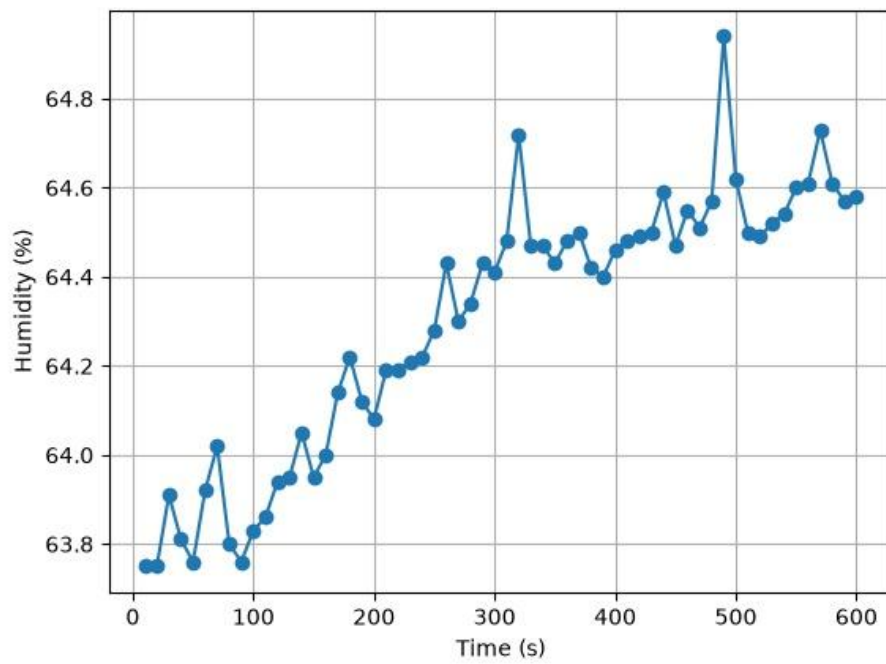
Figure 3: Humidity measurement results
