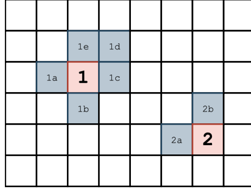
Figure 4: Clustering method for keypoint detection
