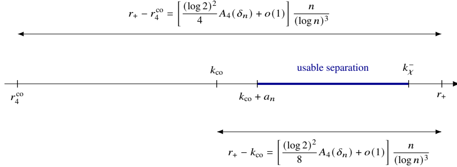
FIGURE 2. Root geometry after rounding and amplification. For all sufficiently large n , r_4^{\text{co}} < k_{\text{co}} < k_{\text{co}} + a_n < k_\chi^- < r_+ . The thick segment is the usable separation; a_n = o(n/(\log n)^3) and r_+ - k_\chi^- \in [\log n, \log n + 2) . The horizontal positions are schematic and not to scale.
