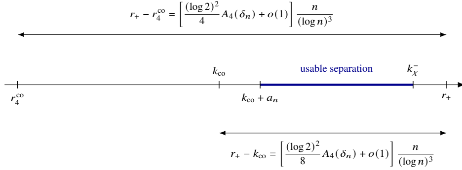
FIGURE 2. Root geometry after rounding and amplification. For all sufficiently large n , r_4^{\text{co}} < k_{\text{co}} < k_{\text{co}} + a_n < k_{\chi}^- < r_+ . The blue interval is the usable separation; a_n = o(n/(\log n)^3) and r_+ - k_{\chi}^- \in [\log n, \log n + 2) . The horizontal positions are schematic and not to scale.
