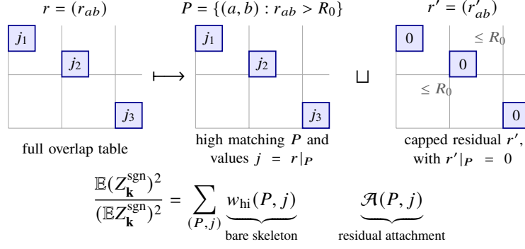
FIGURE 1. Canonical high-cell extraction, shown on a schematic overlap table. Highlighted cells lie in distinct rows and columns and therefore form a matching. Proposition 9.1 proves the finite bijection and the displayed normalized factorization.
