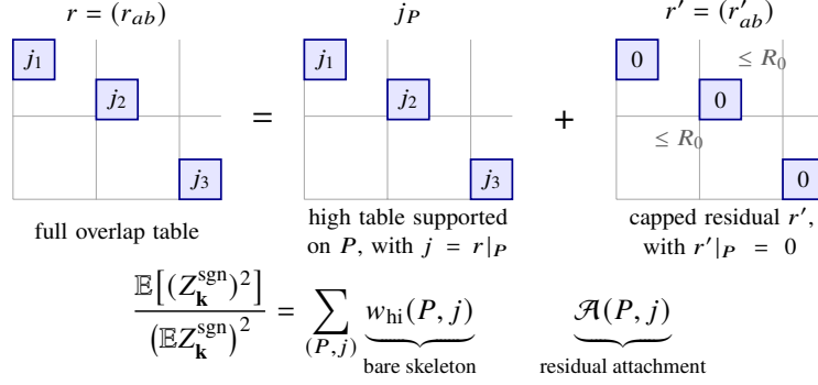
FIGURE 2. Canonical high-cell extraction at the overlap-table level. The highlighted cells P = \{(a, b) : r_{ab} > R_0\} form a matching and have multiplicities j = r|_P ; extending j by zero off P gives r = j_P + r' , where the capped residual table r' vanishes on P . Unlabeled cells of the first panel are unrestricted table entries; they are zero off P in j_P and at most R_0 off P in r' . Proposition 9.1 (where Section 9 writes M = P ) lifts this table decomposition to a bijection of labeled configuration matchings by retaining both the selected-pair set S \in \mathfrak{F}(P, j) and the residual matching \Pi_{\text{res}} , and yields the displayed normalized factorization.
