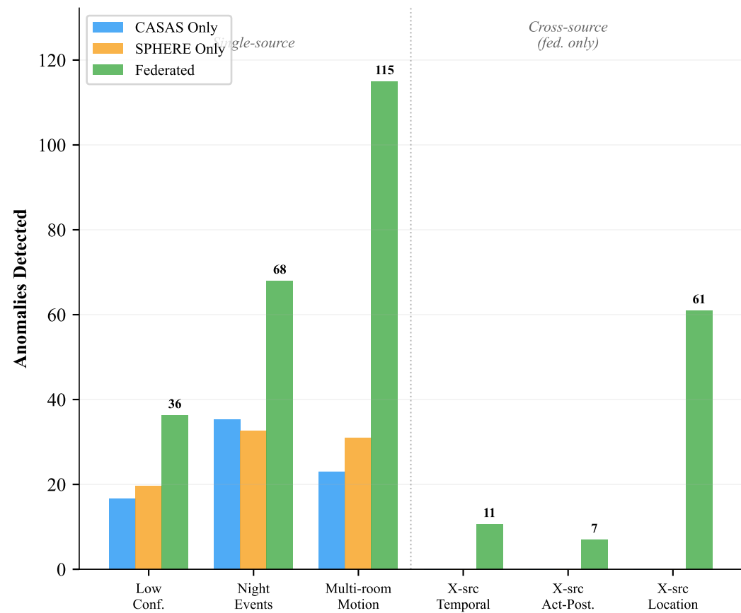
(a) Anomaly Detection: Single vs. Federated
