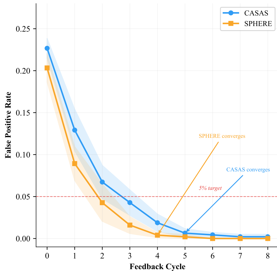
(b) False Positive Rate vs. Feedback Cycle
