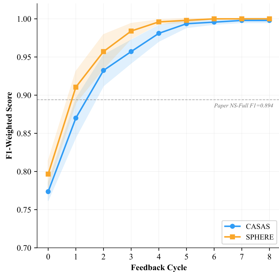
(a) F1-Weighted Score vs. Feedback Cycle
