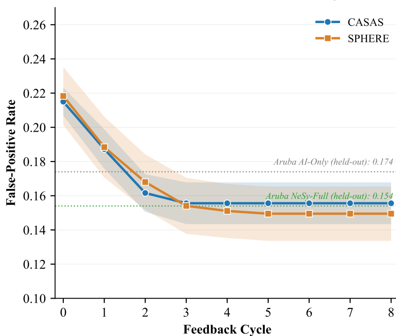
(b) False-Positive Rate vs. Feedback Cycle
