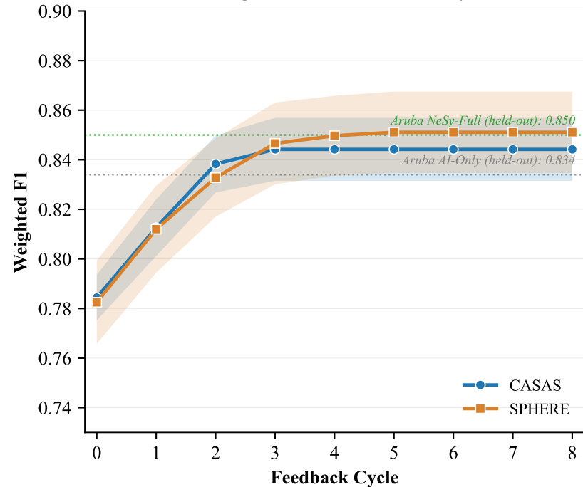
(a) Weighted F1 vs. Feedback Cycle
