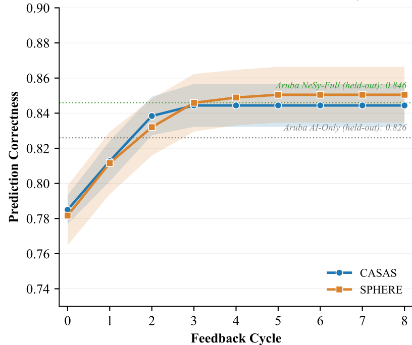
(c) Prediction Correctness vs. Feedback Cycle
