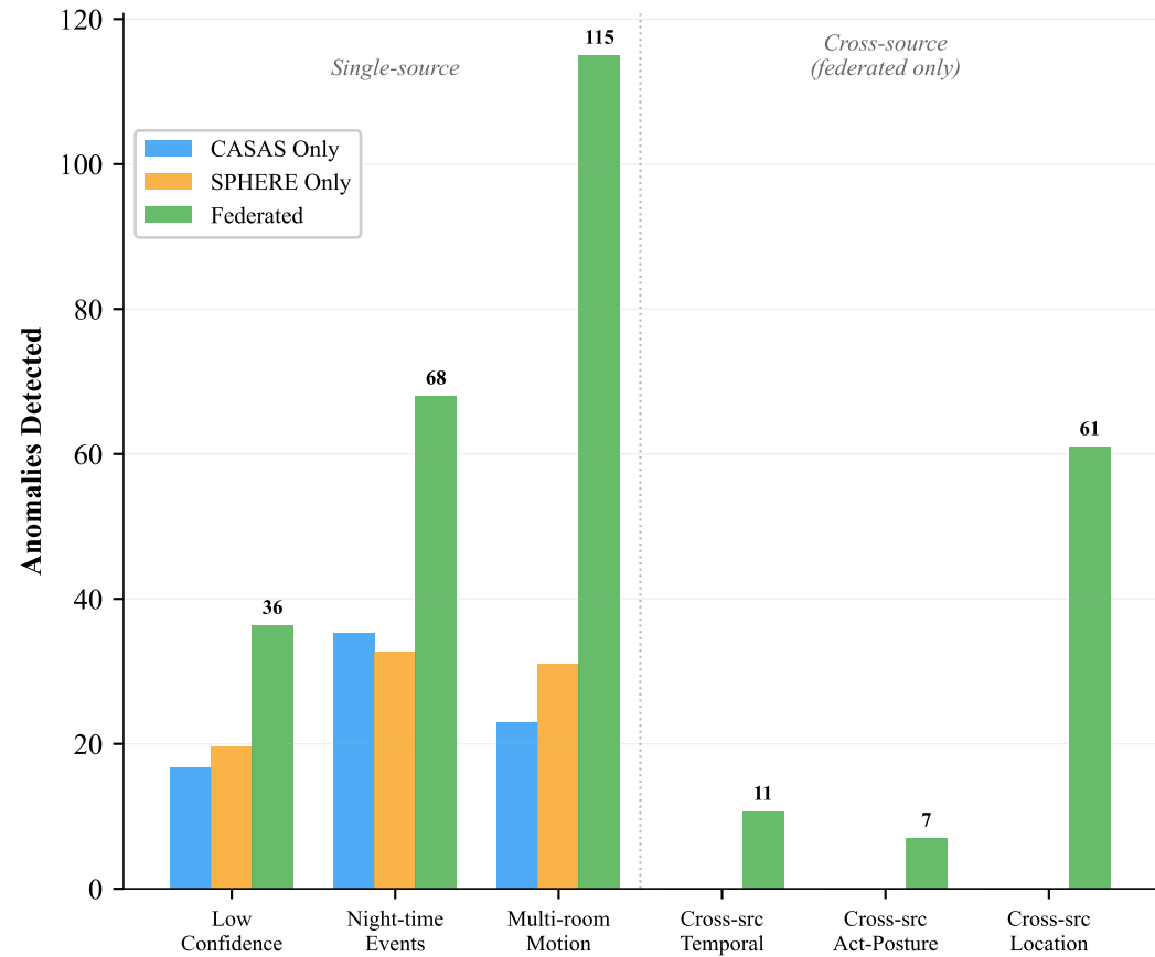
(a) Anomaly Detection: Single-Source vs. Federated
