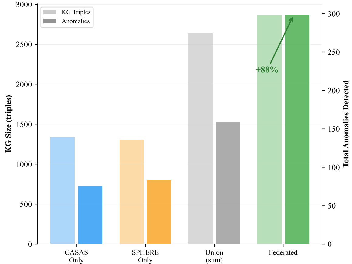
(b) KG Size and Detection Coverage
