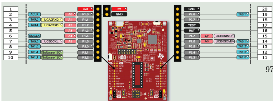
Figure 3.8.: MSP-EXP430G2ET Pinout Diagram
