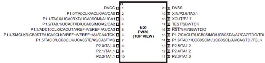
Figure 7.19.: The 20-pin MSP430G2553 pinout identifies the alternative peripheral functions available on each GPIO pin.
