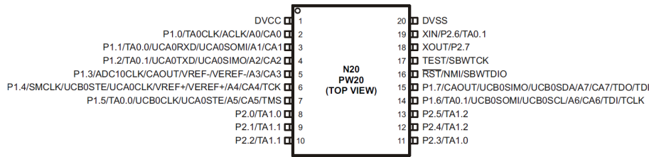
Figure 3.7.: MSP430G2553 Pinout Diagram
