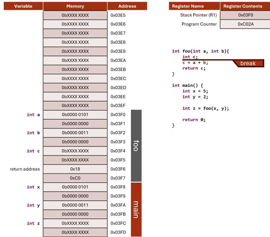
Figure 2.7.: Example C code and the condition of the stack up to the indicated break point. “X” indicates bit values that have been uninitialized.
