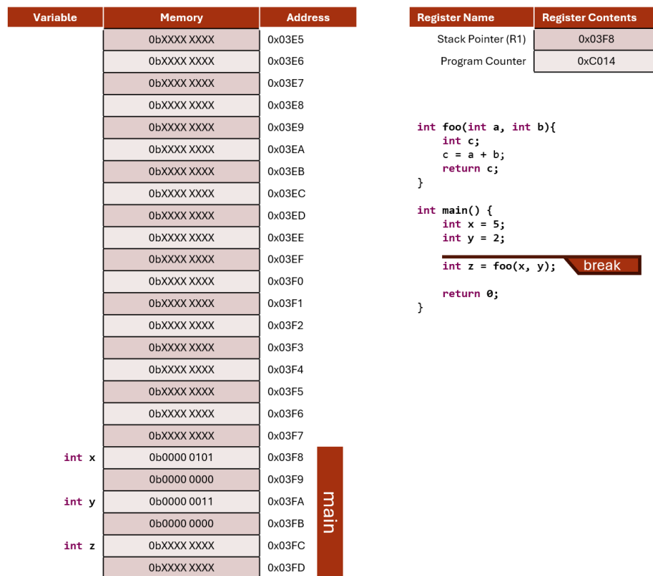
Figure 2.6.: Example C code and the condition of the stack up to the indicated break point. “X” indicates bit values that have been uninitialized.
