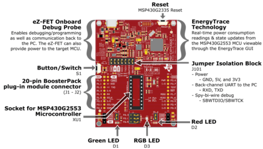
Figure 2. MSP-EXP430G2ET Overview
