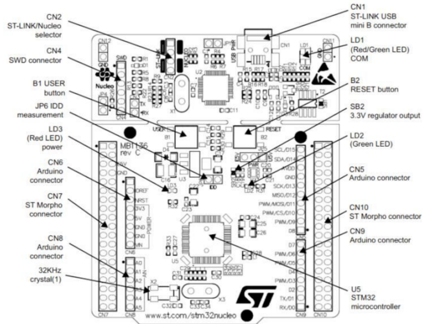
Figure 1.3.: An overview of the STM32 Nucleo-64 development board. (Source: STMicroelectronics, UM1724 STM32 Nucleo-64 boards user manual.)
