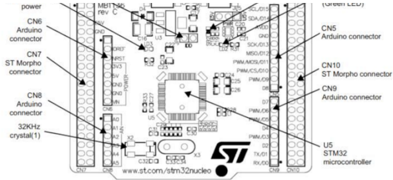
Figure 1.4.: The STM32F091RC microcontroller (U5) and the surrounding Arduino-compatible (CN5, CN6, CN8, CN9) and ST Morpho (CN7, CN10) breakout headers that give access to its pins. (Source: STMicroelectronics, UM1724 STM32 Nucleo-64 boards user manual.)
