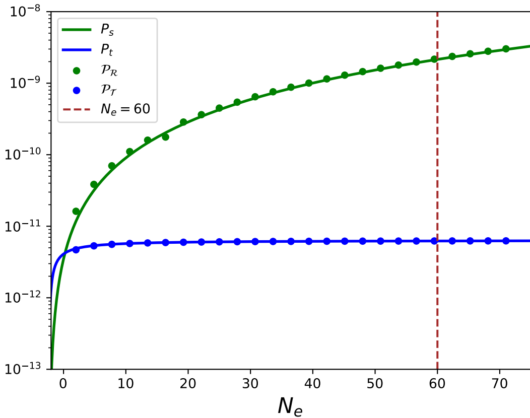
Super-Hubble Power Spectra
