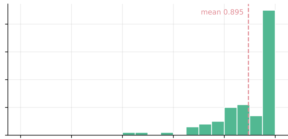
K2-Horizon 36B
