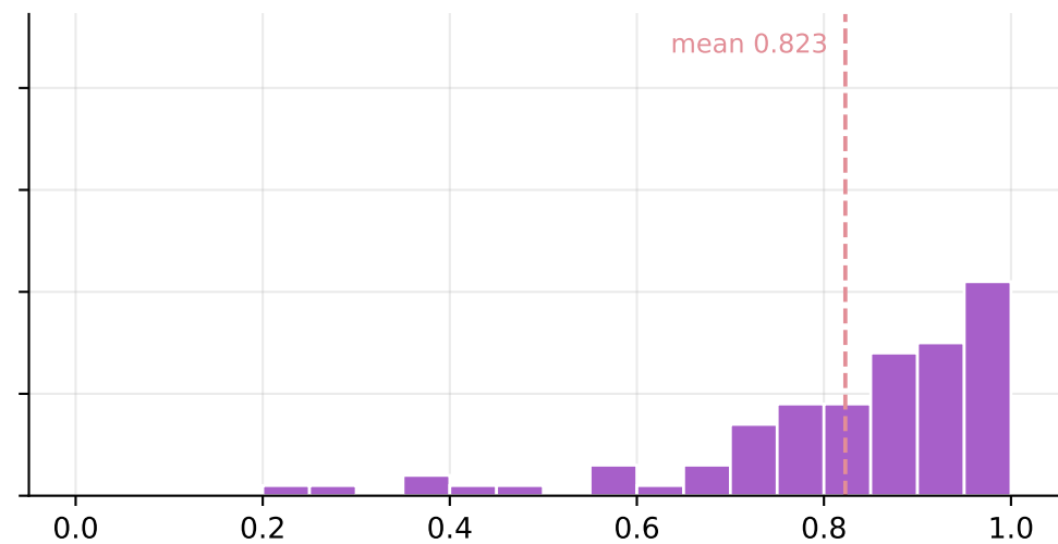
K2-Horizon 4B
