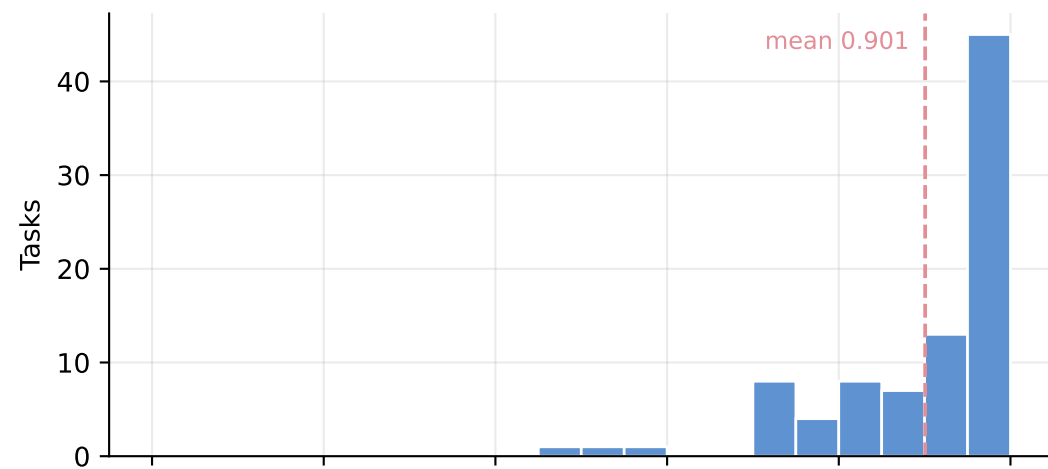
K2-Horizon
