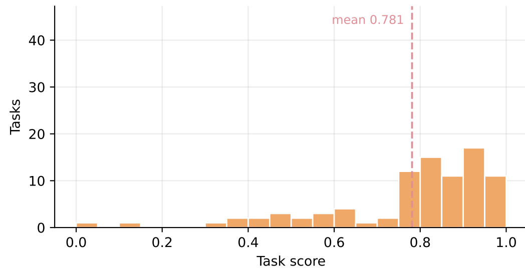
K2-Horizon 1B
