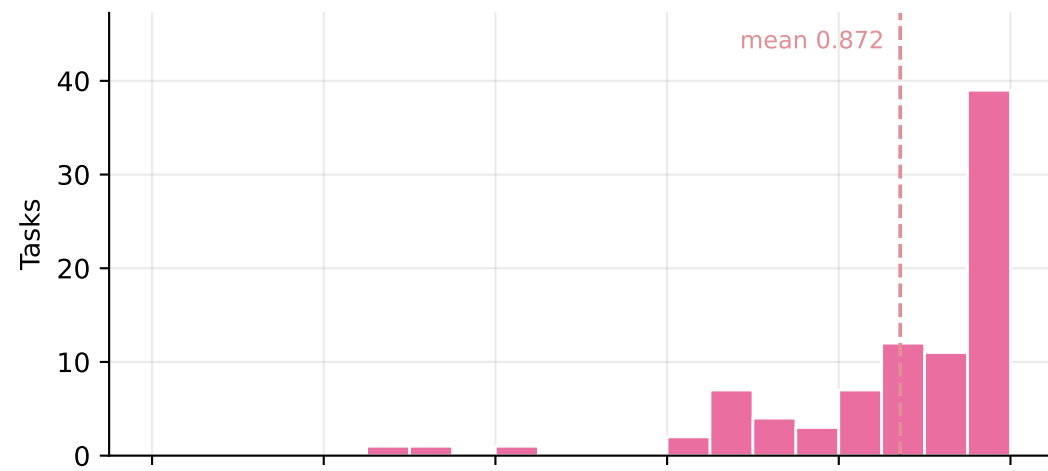
K2-Horizon 7B
