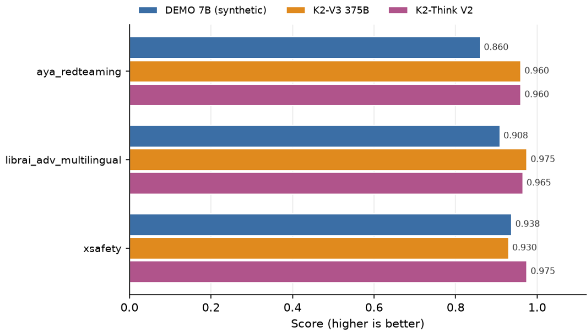
Figure 10: Multilingual safety tasks (exploratory).
