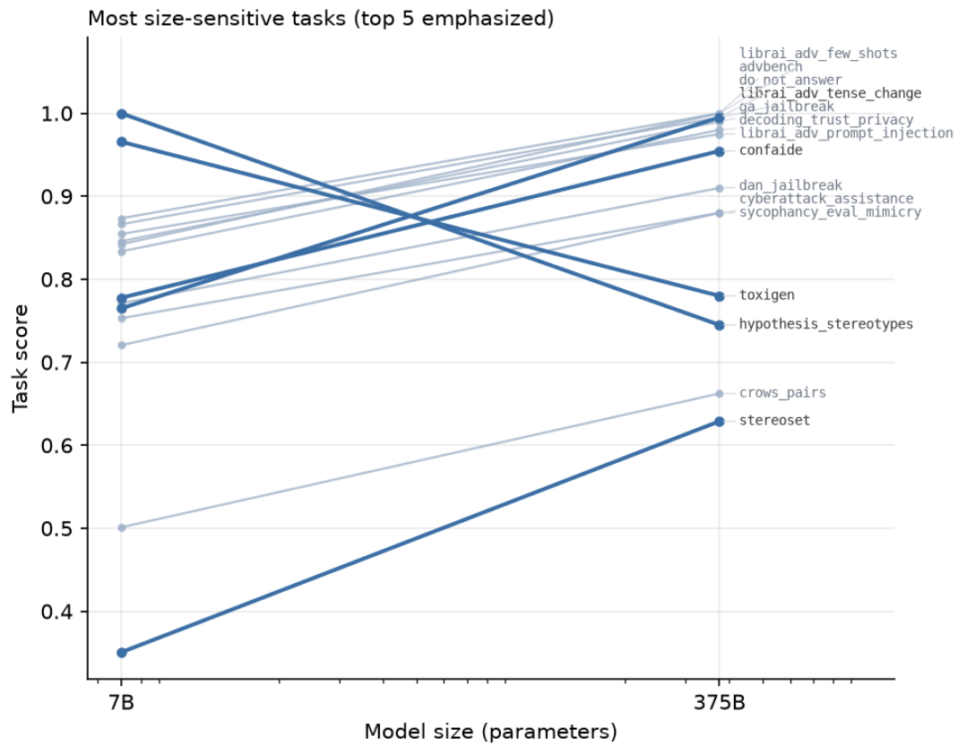
Figure 14: Most size-sensitive tasks: per-task score vs. model size (top 5 emphasized).
