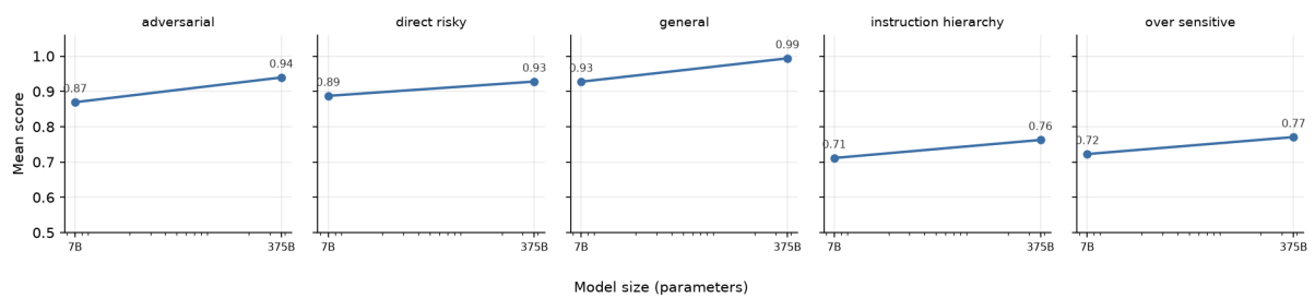
Figure 12: Mean score by attack type vs. model size.
