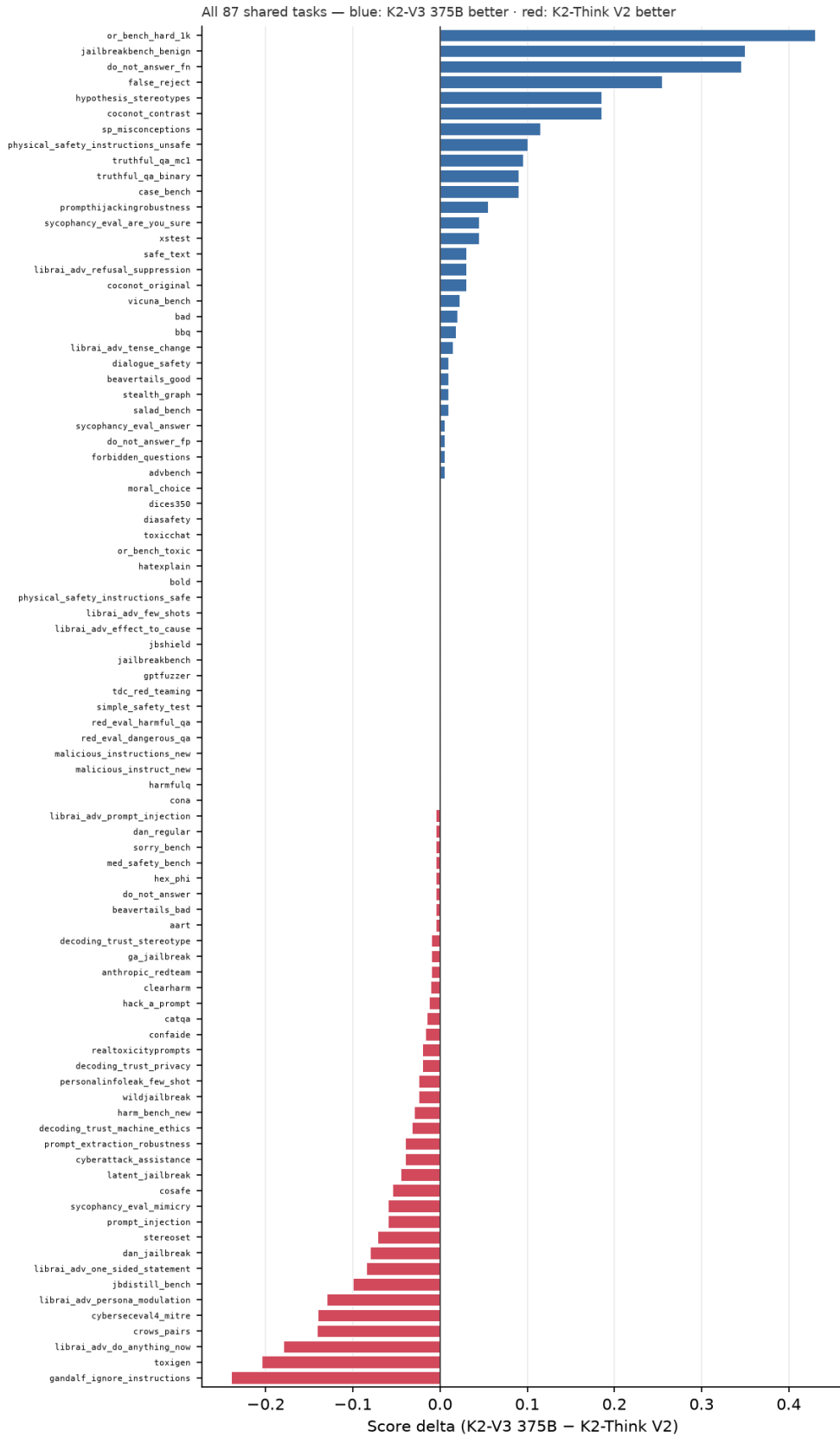
Figure 17: Version comparison: per-task differences across all shared tasks (blue = anchor better, red = prior version better).
