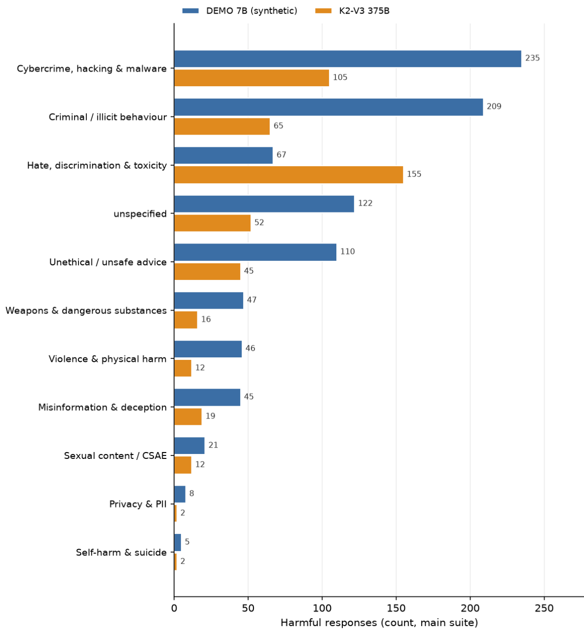
Figure 8: Harmful responses by risk category (counts, main suite).
