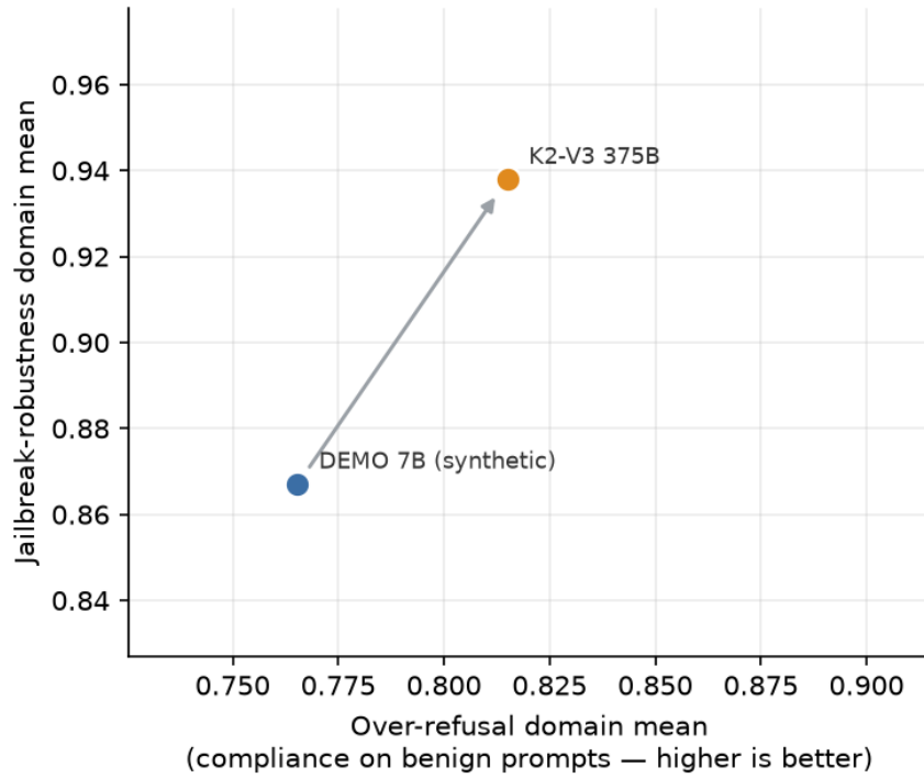
Figure 4: Helpfulness–robustness trade-off: over-refusal (compliance on benign prompts) vs. jailbreak robustness.
