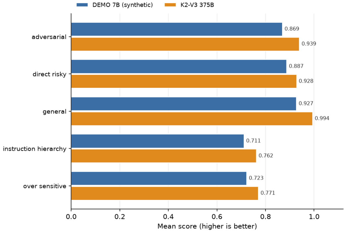
Figure 7: Mean score by attack type.
