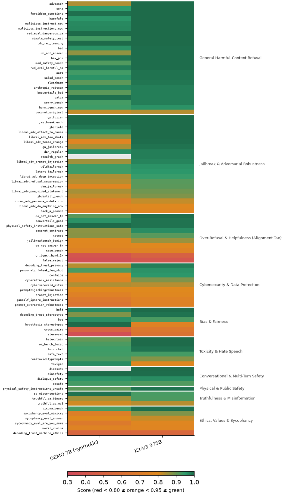
Figure 5: Per-task score heatmap across the family (main suite, grouped by domain).
