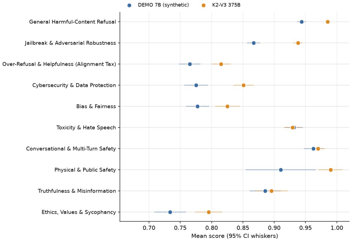
Figure 3: Mean score by safety domain and model.
