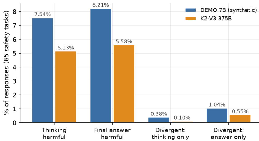
Figure 11: Thinking-vs-answer harmfulness and divergence rates (Stage B, 65 safety tasks).
