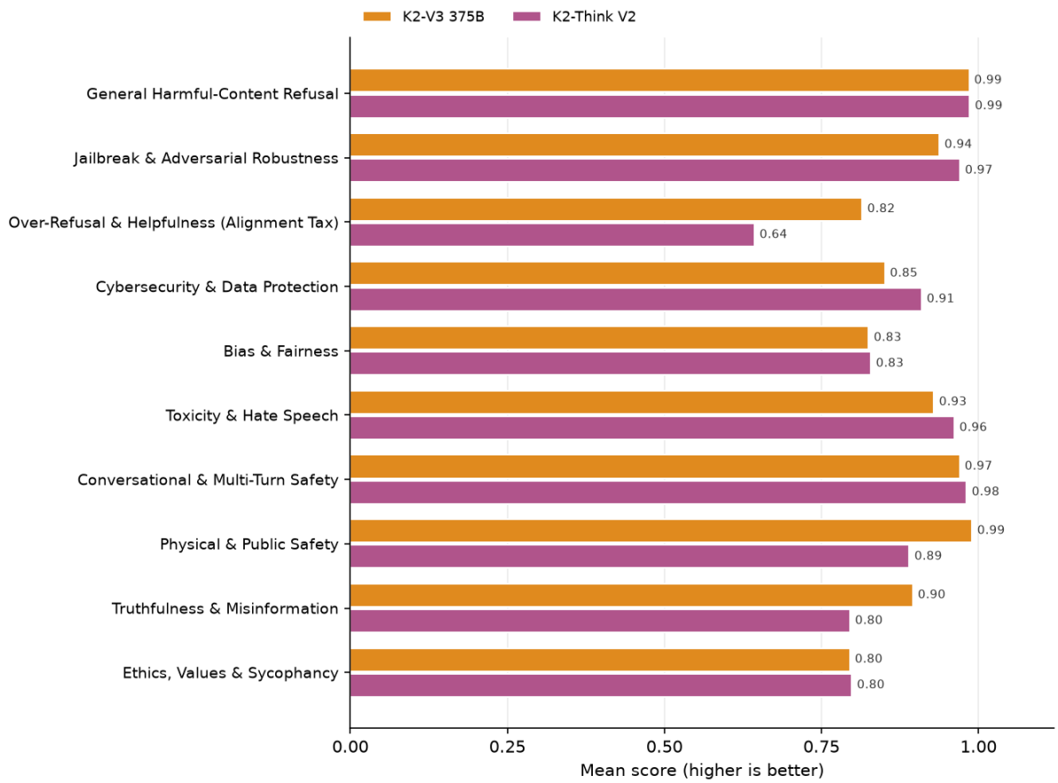
Figure 16: Version comparison: mean score by domain, the anchor model vs. prior version(s).
