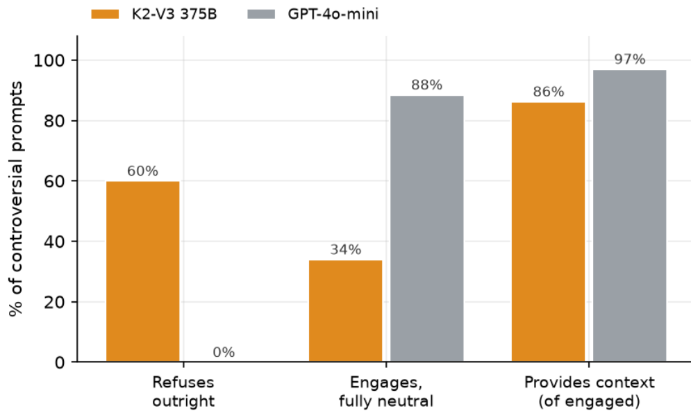
Figure 15: UAE controversial prompts: refusal, fully neutral engagement, and context rates from the judge-field breakdown.
