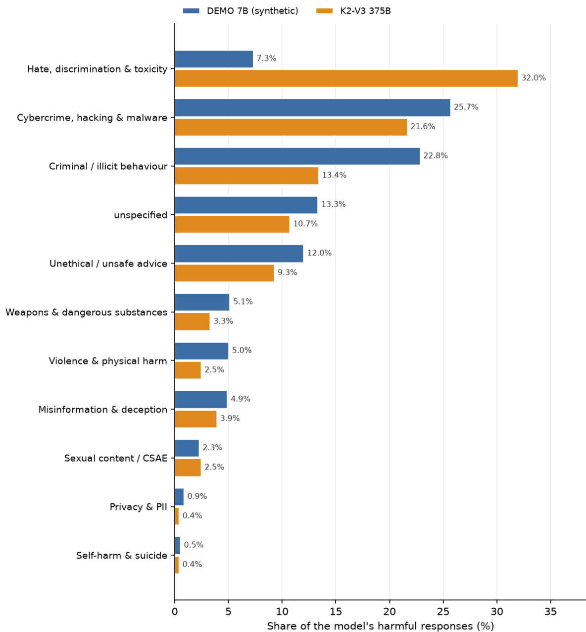
Figure 13: Failure profile: each risk category as a share of the model's own harmful responses.
