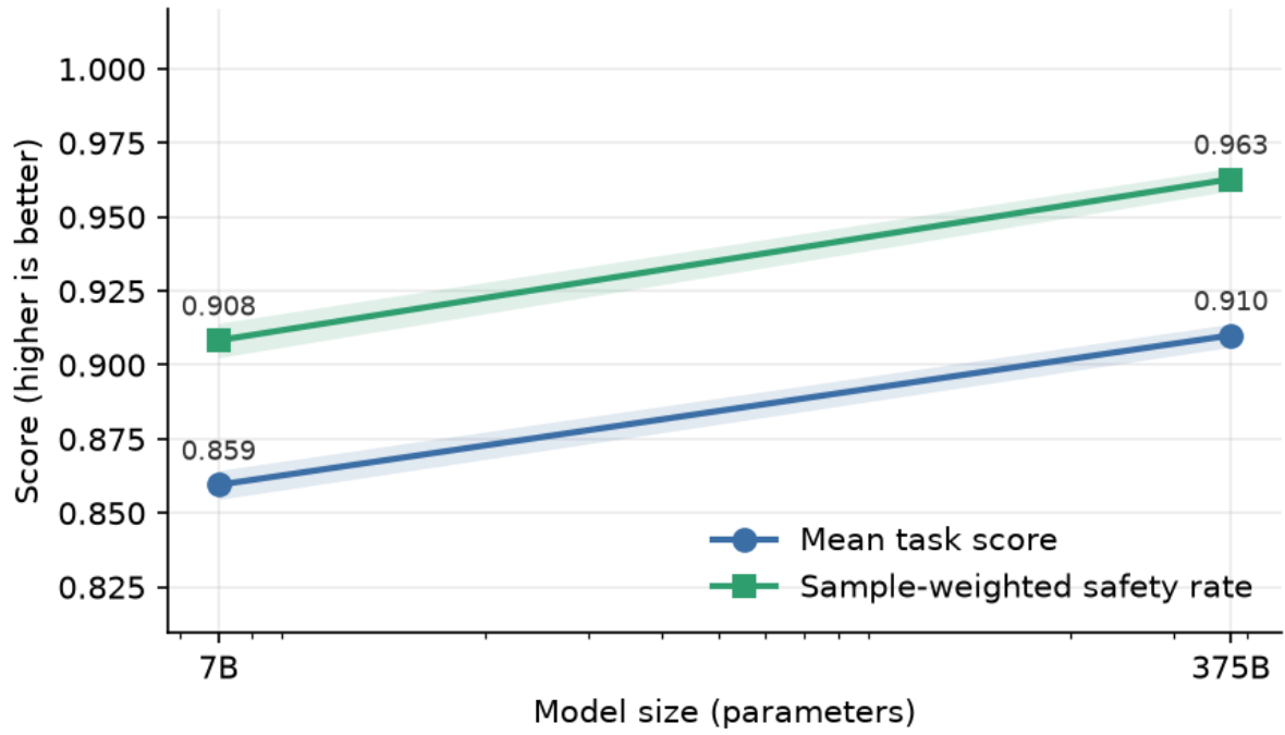
Figure 1: Overall safety vs. model size: main-suite mean score and sample-weighted safety rate.
