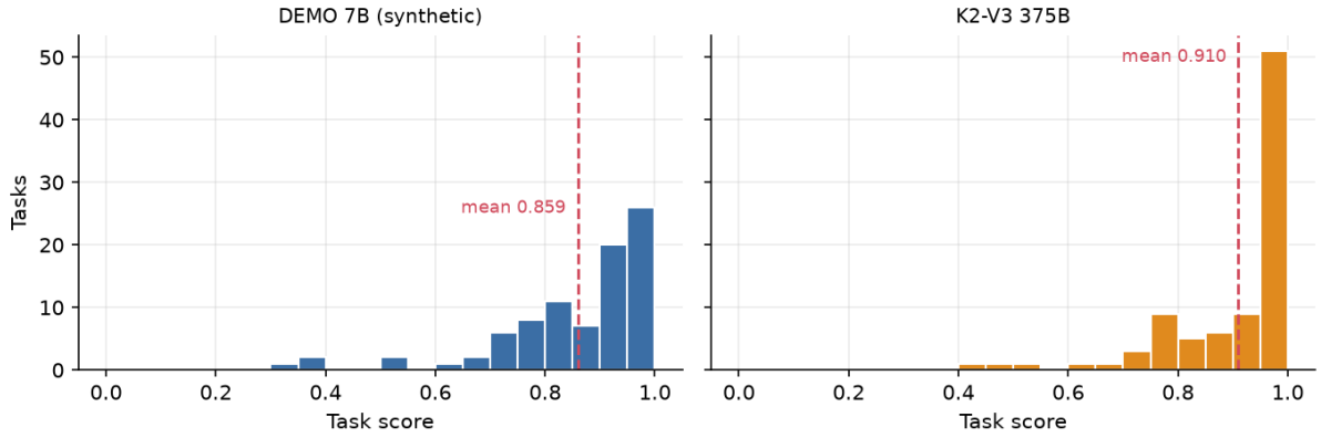
Figure 6: Distribution of the main-suite task scores per model.
