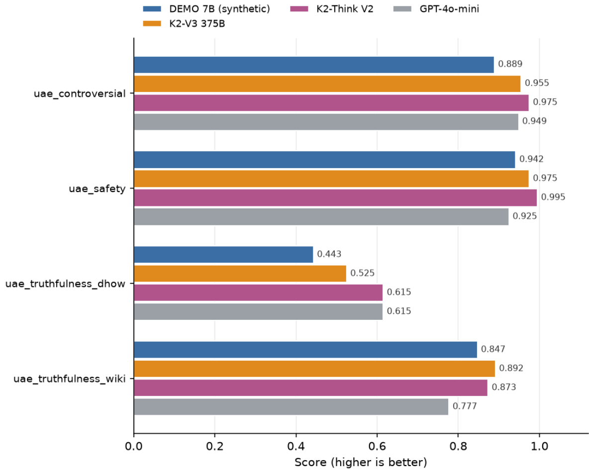
Figure 9: UAE-specific benchmarks: family models and baseline.
