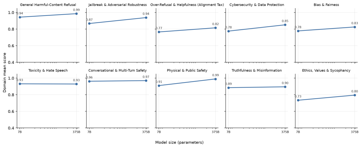
Figure 2: Per-domain mean score vs. model size.
