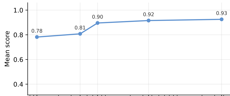
Adversarial
