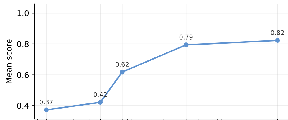
General
