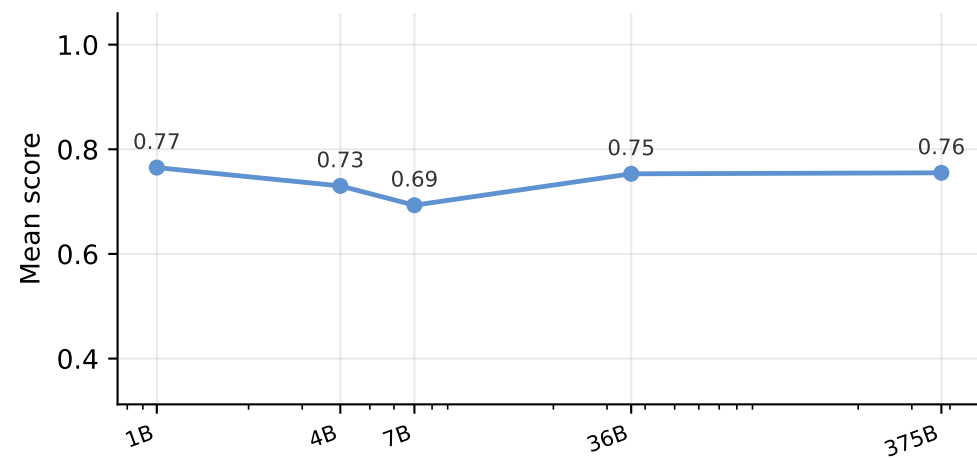
Over-sensitive
