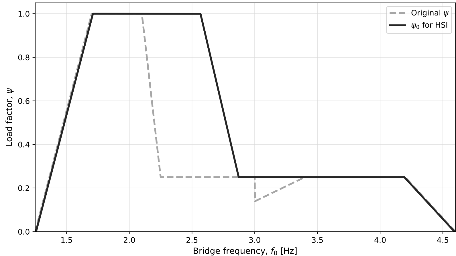
\psi of EN1990 and proposed \psi to contain HSI
