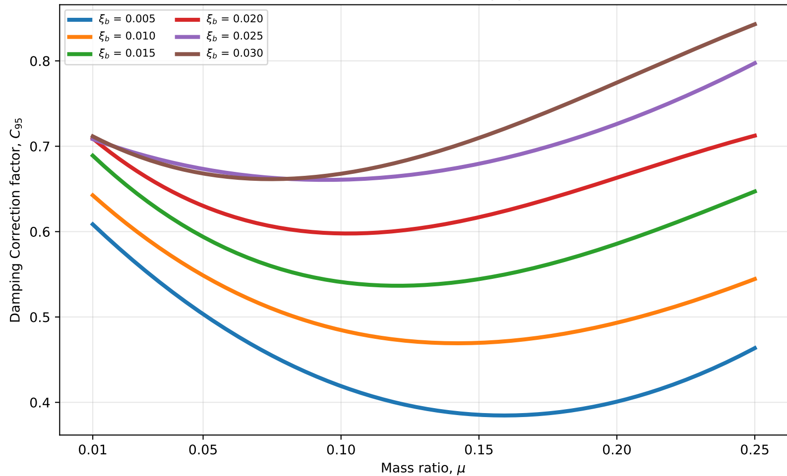
Idealization of P95 Bias for damping correction
