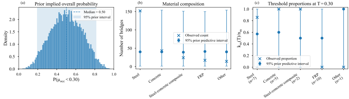
Figure 7: Prior predictive assessment of the pedestrian-to-structure mass-ratio probability model at T = 0.30 : (a) prior-implied distribution of the overall probability P(\mu_{\text{occ}} < 0.30) ; (b) prior predictive intervals for the material composition of the bridge population compared with the observed material counts; and (c) prior predictive intervals for the material-specific threshold proportions k_m(T)/n_m compared with the observed proportions.
