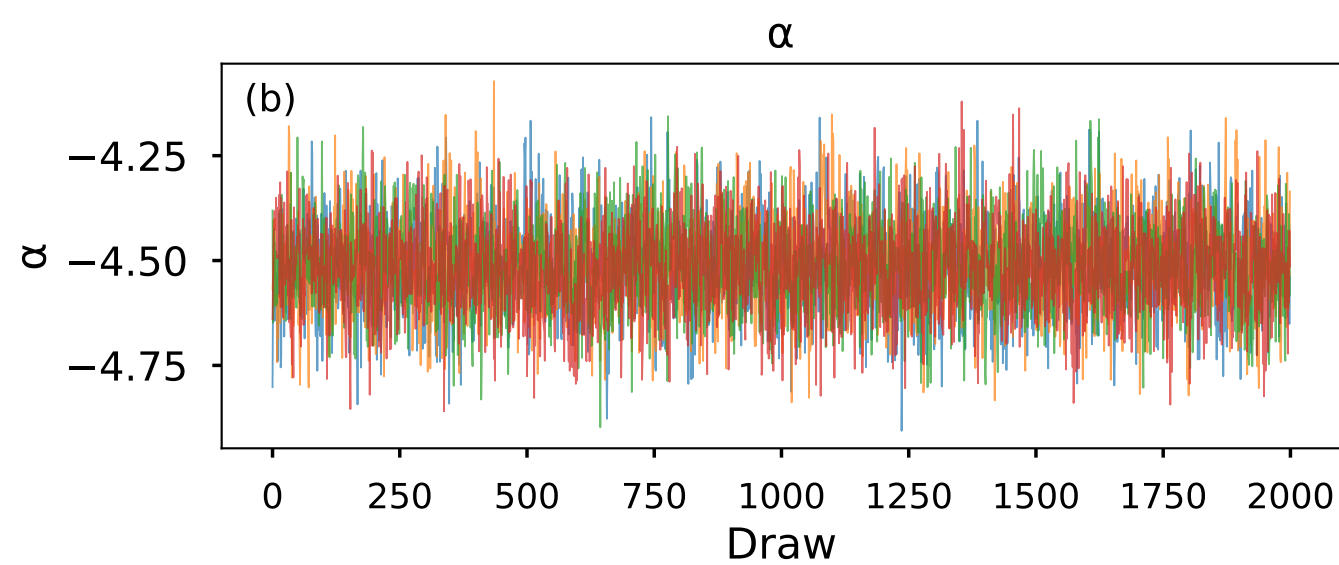
Trace plots
