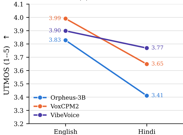
(b) Naturalness
