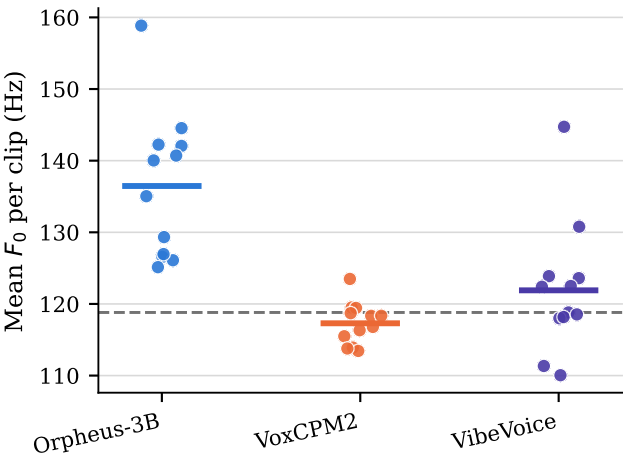
Pitch register vs. the reference voice
