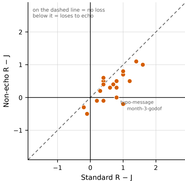
Qwen3.5-27B
