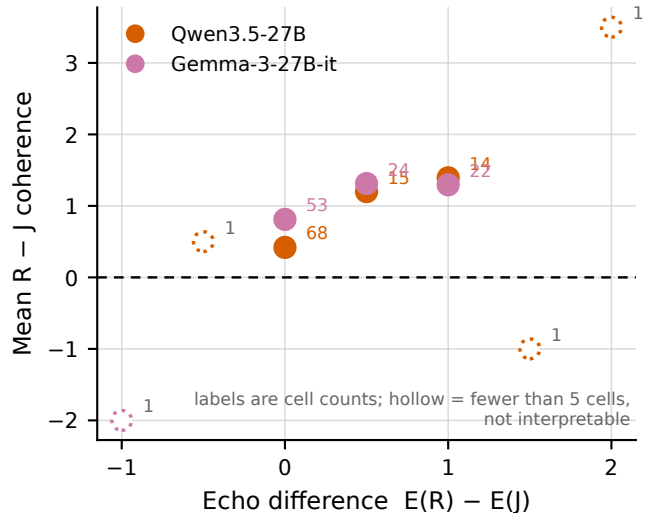
b By echo difference
