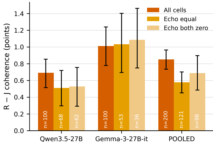
a Effect under echo restriction
