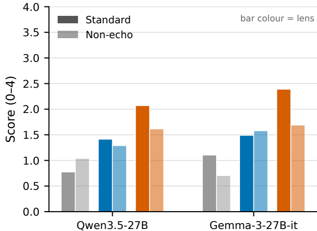
a Mean score: standard vs non-echo
