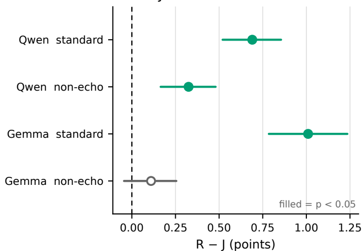
b R - J under each rubric
