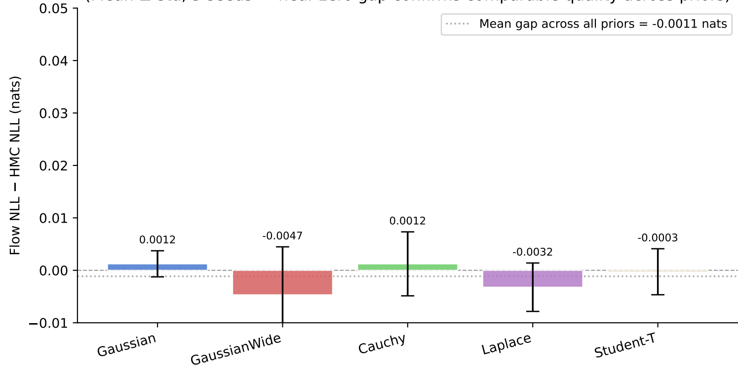
Flow Matching Approximation Error vs HMC Reference (Mean \pm std, 5 seeds — near-zero gap confirms comparable quality across priors)
