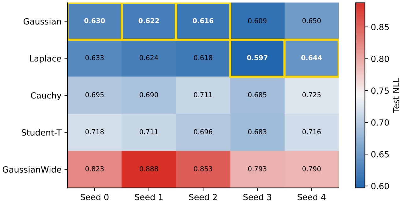
Test NLL per Prior per Seed (German Credit, n = 75 , lower = better)
