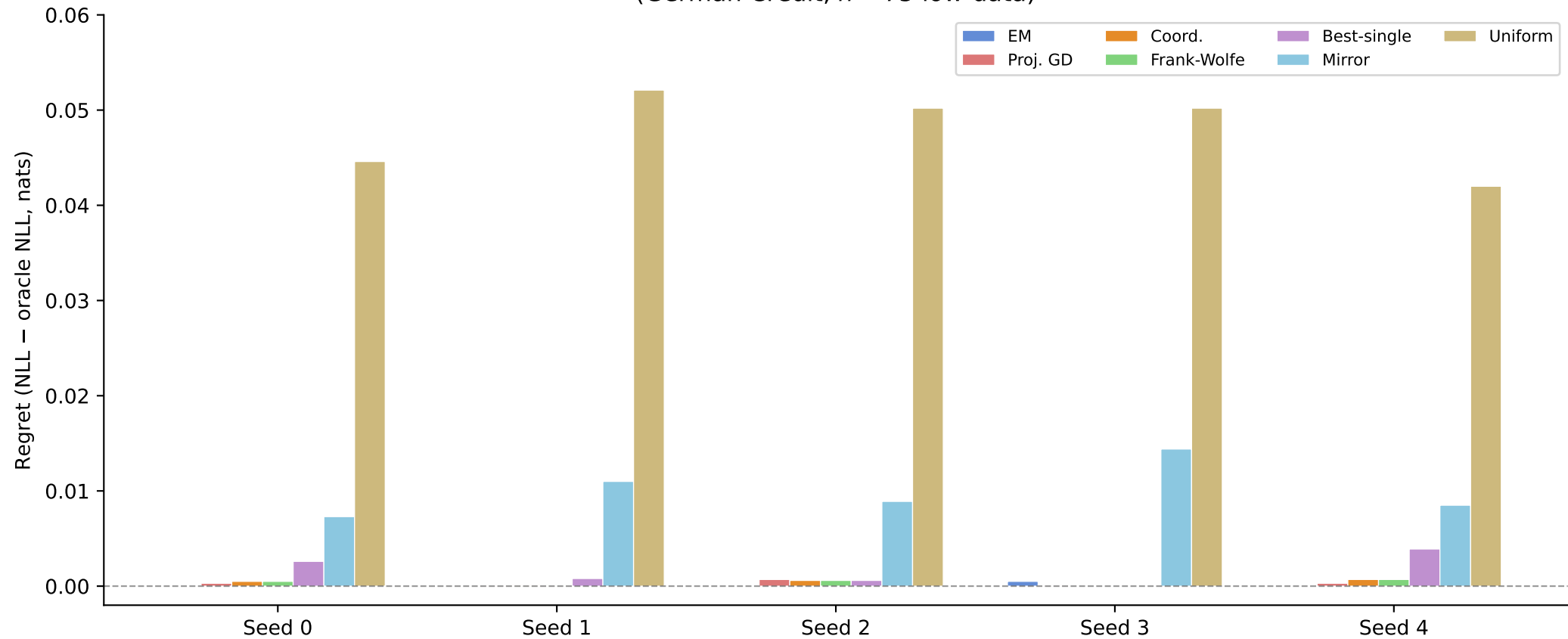
Regret per Seed: All Weight Optimisation Algorithms (German Credit, n = 75 low-data)
