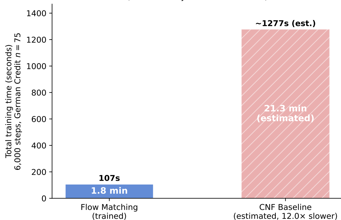
Estimated Total Training Time (same VelocityResNet architecture)
