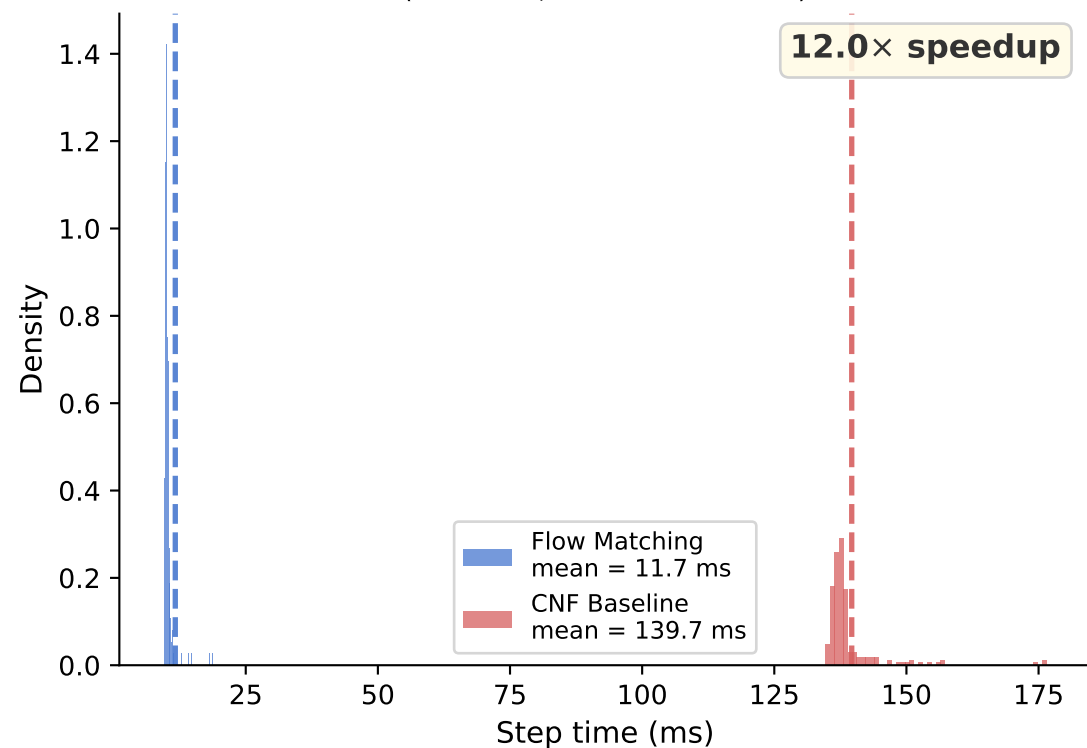
Per-Step Training Time Distribution (200 trials, same architecture)
