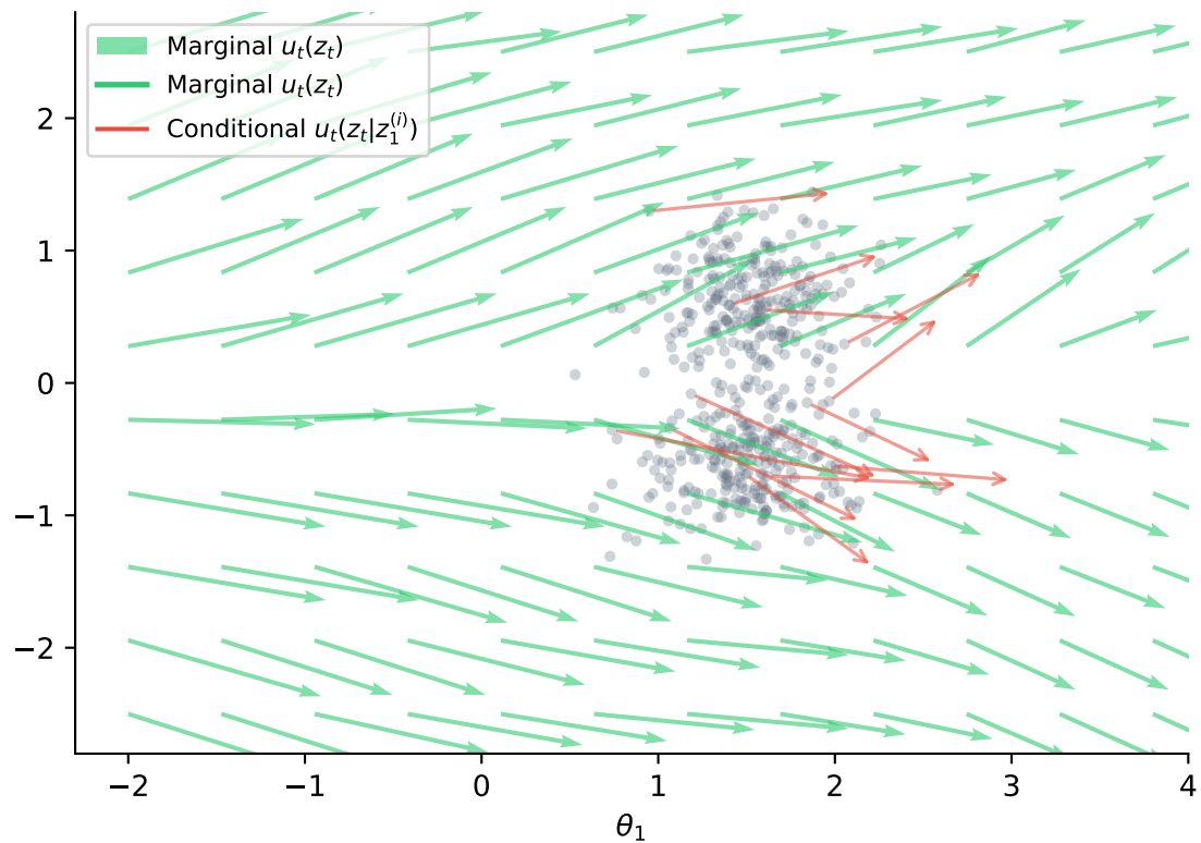
t = 0.6 : Marginal vs Conditional Velocity
