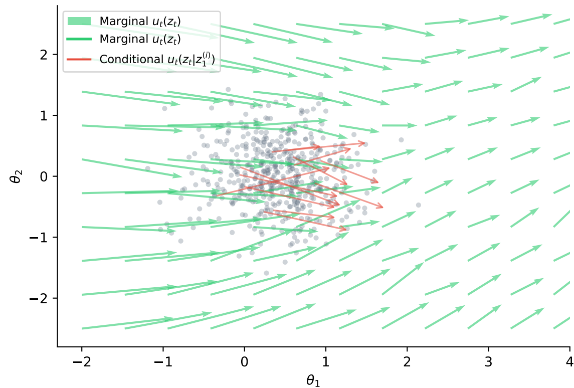
t = 0.15 : Marginal vs Conditional Velocity
