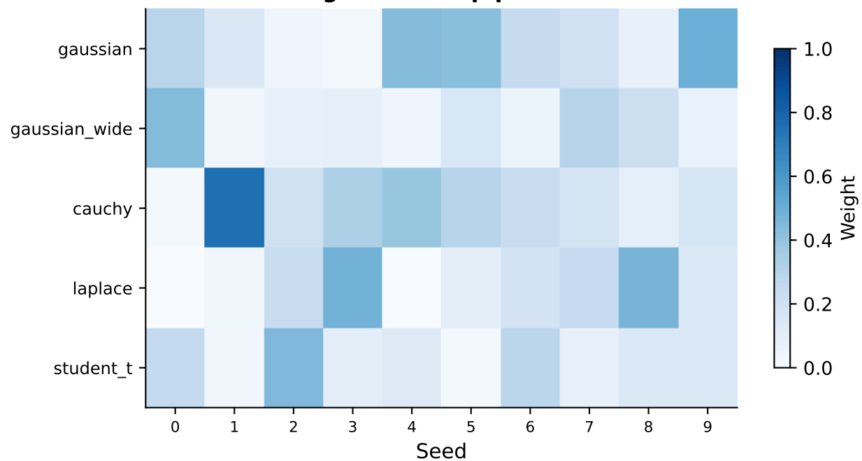
Weight Heatmap per Seed
