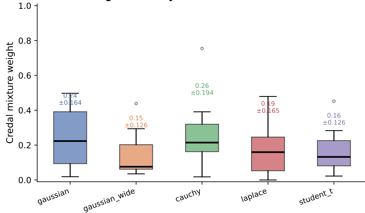
Weight Stability Across 10 Random Seeds
