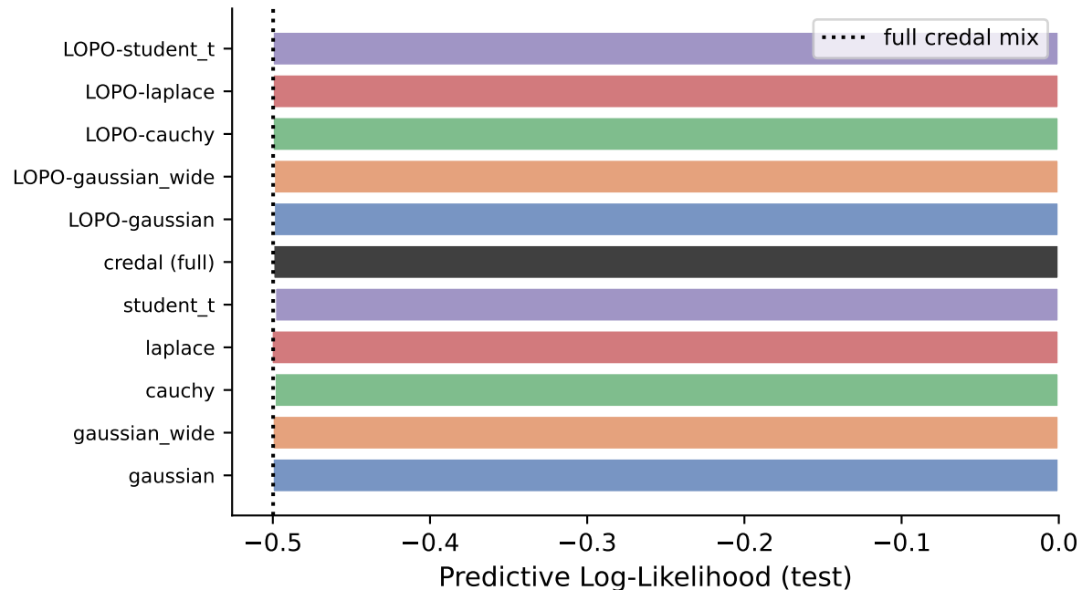
Absolute Pred-LL: Single / LOPO / Full
