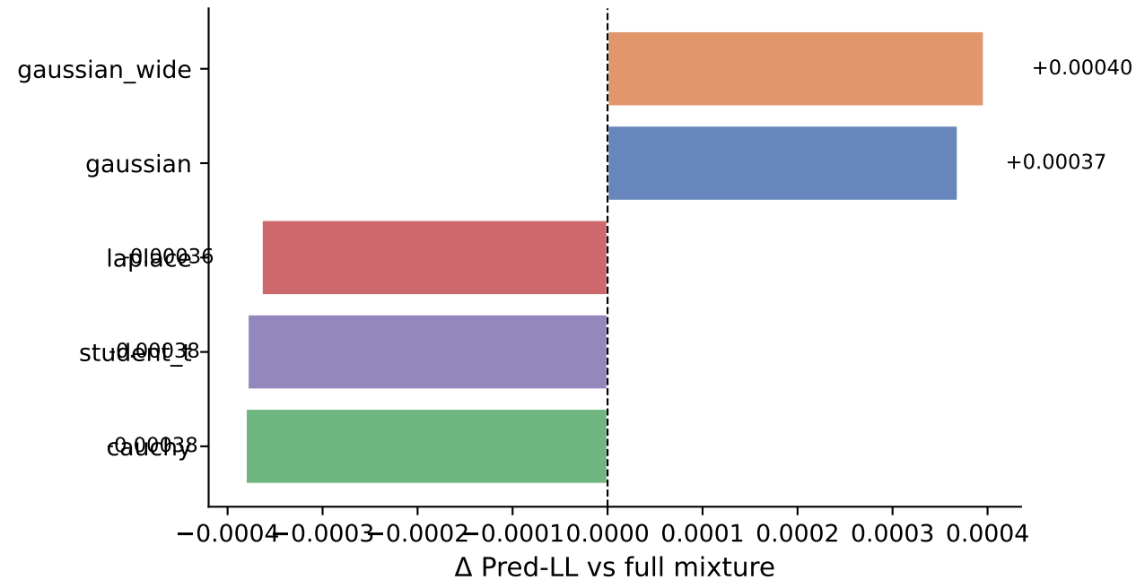
LOPO: Drop in Performance When One Prior Is Removed
