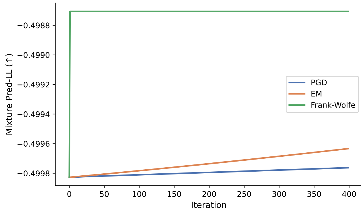
Convergence of Credal Objective (All Optimisers Reach Similar Solution)
