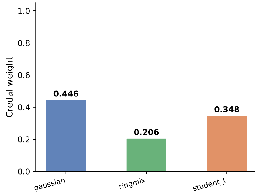
A — Optimised Mixture Weights
