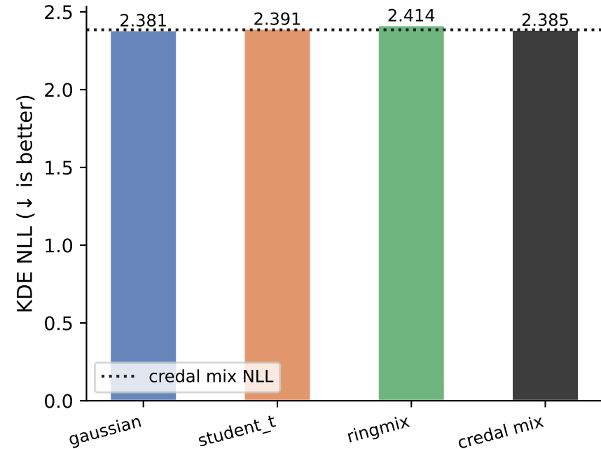
C — Absolute NLL: Single vs Mixture
