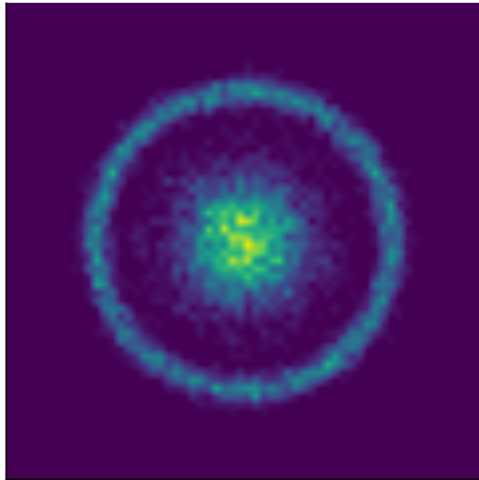
Ground Truth
