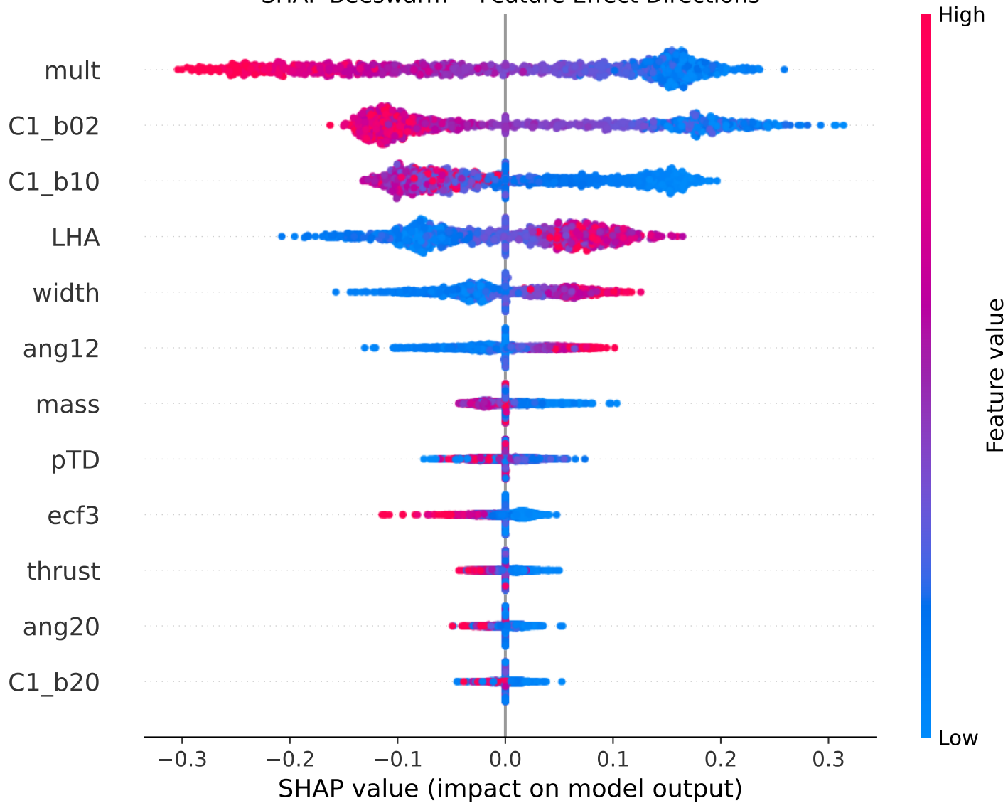
SHAP Beeswarm -- Feature Effect Directions
